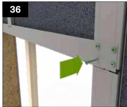
Ensuring the tray is level and propped at the centre (prop NOT SUPPLIED), fix the tray into the walling panel clips at both ends with four GPHS fixings and for each walling panels on the tray with two GPHS fixings through the pre punched holes.
