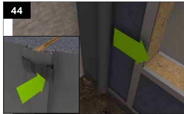
Unroll the membrane over the walls allowing this to sit slightly below DPC level (around 10 mm). Ensure that any joins in the membrane overlap by a minimum of 100mm horizontally and 150mm vertically. This can be clipped in place using the membrane clips provided. The membrane detail at the top of the wall is shown at the beginning of each roof beam installation section.
